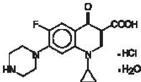
Figure 1: Structure of Ciprofloxacin
